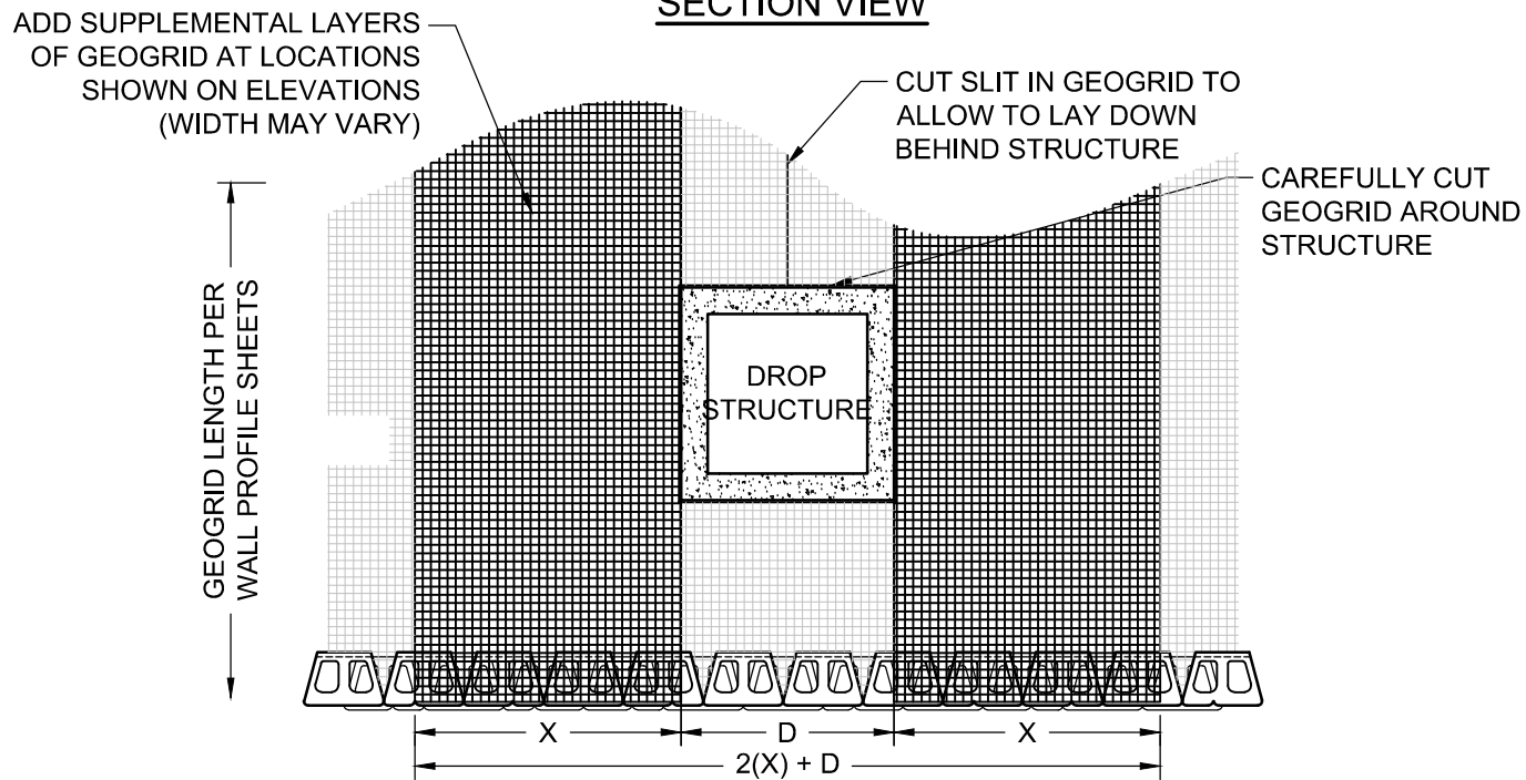
PLAN VIEW
