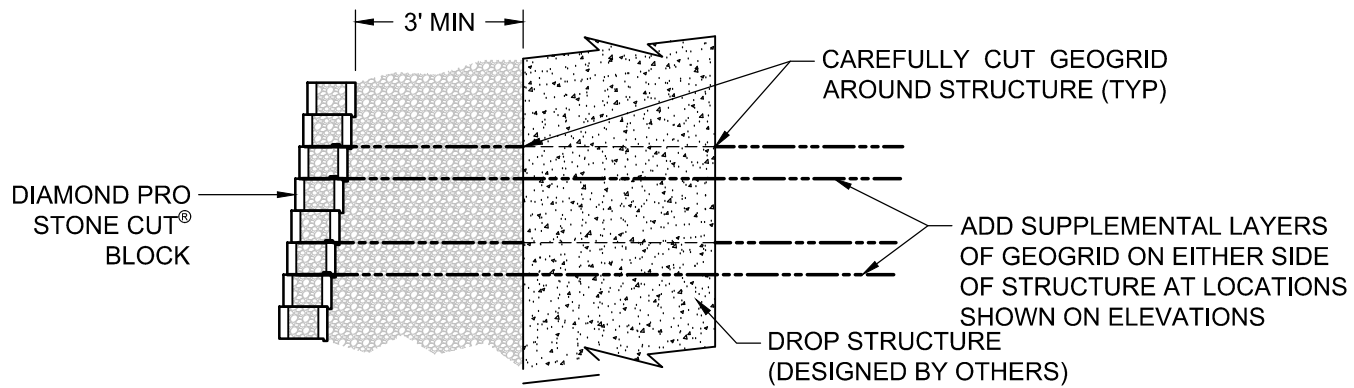
SECTION VIEW
