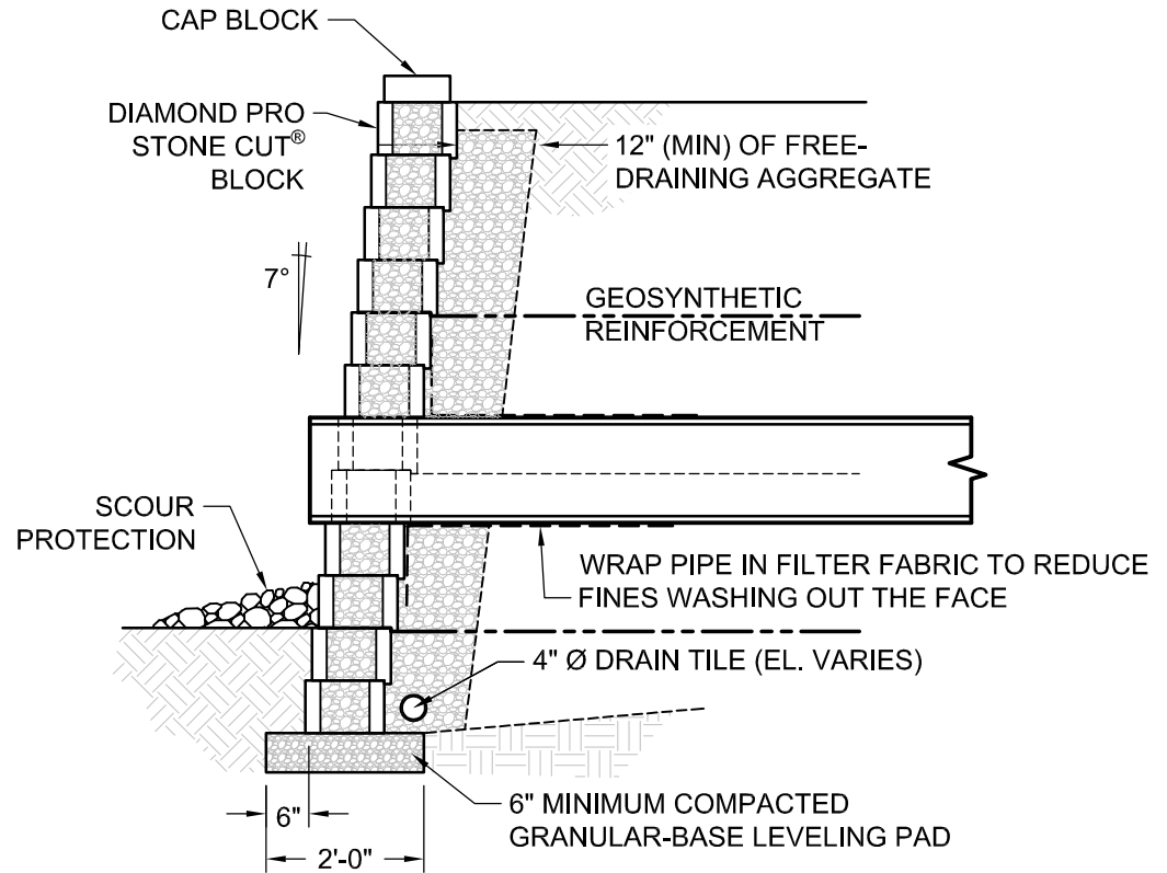
SECTION VIEW
