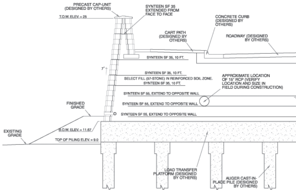
Typical wall section. This image represents half of land bridge detail.
