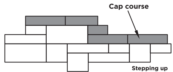
Stepping up
