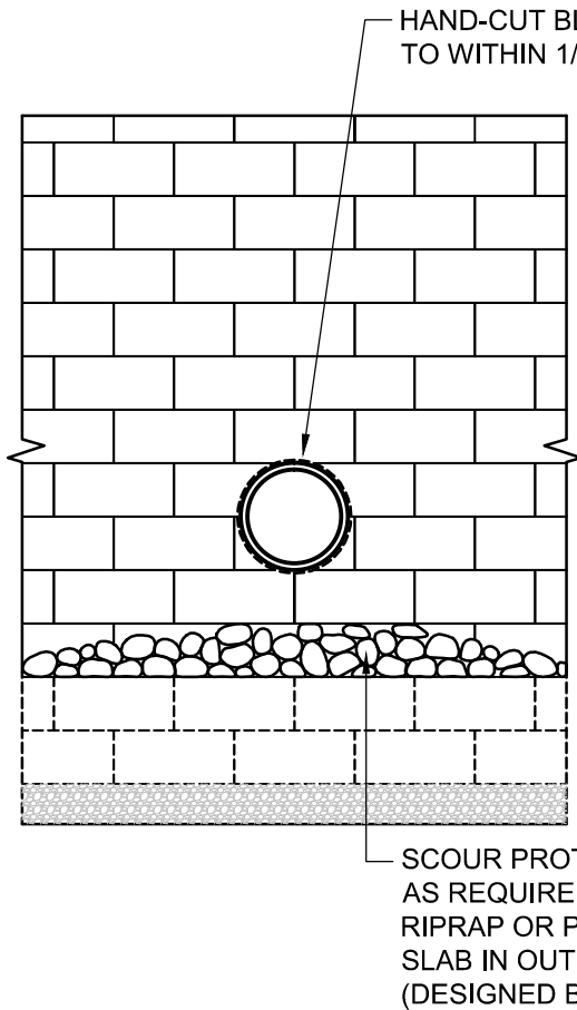
ELEVATION VIEW
