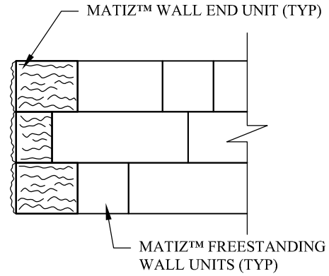
ELEVATION VIEW
