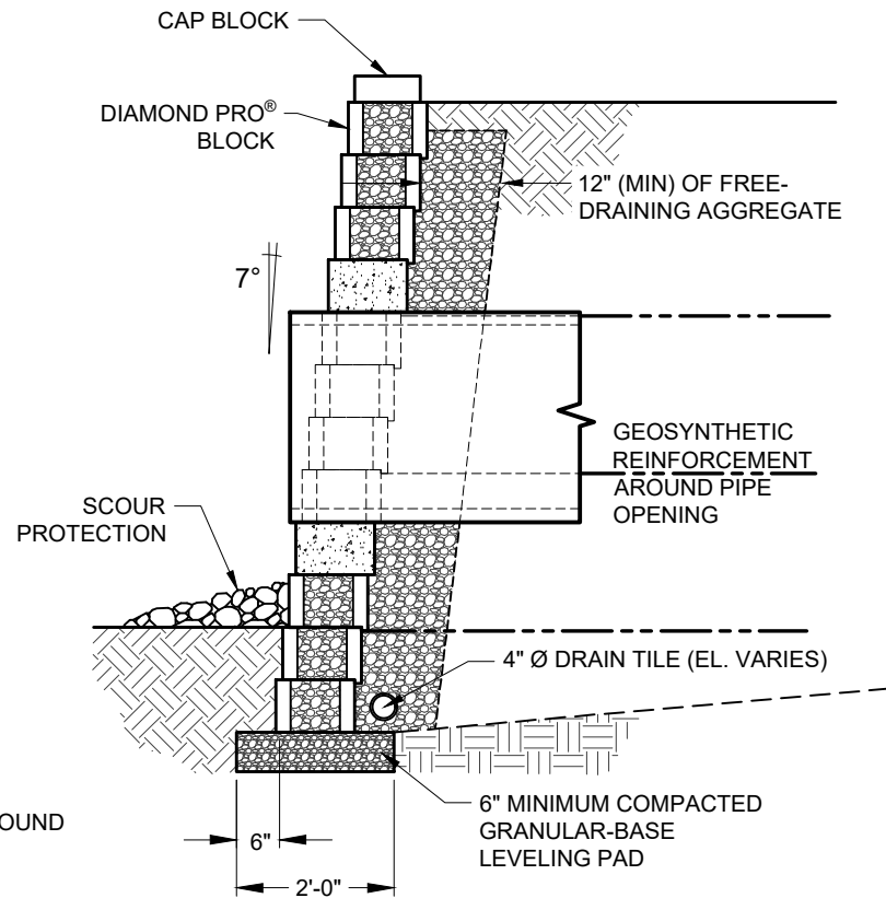
SECTION VIEW
