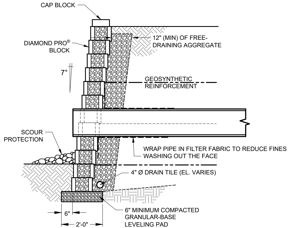
SECTION VIEW
