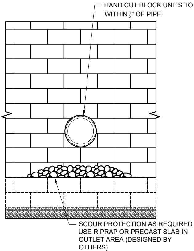
FACE VIEW
